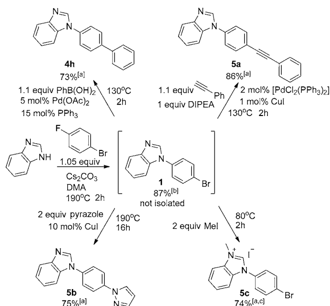
Scheme 2. Scope of one-pot reactions. [a] Yield of isolated product (after 2 steps). [b] Determined by HPLC. [c] Trifluoroacetate salt after purification.
