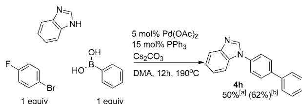
Scheme 3. Simultaneous S_NAr substitution and cross-coupling. [a] Yield of isolated product. [b] Yield corrected for unconverted benzimidazole.
